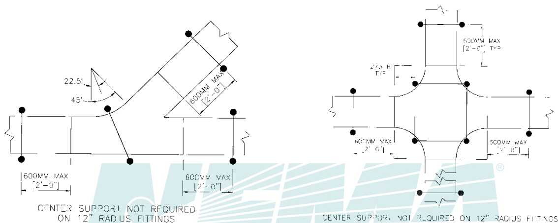
Figure 3-56 Horizontal Wye
