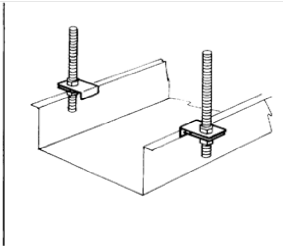
Figure 3-11 Double Cable Tray Hanger
