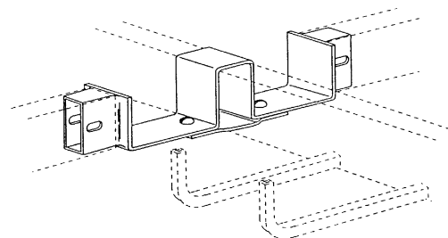
Figure 3-51 Horizontal Cross Connector
