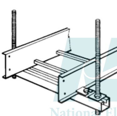
Figure 3-3 Strut Support
