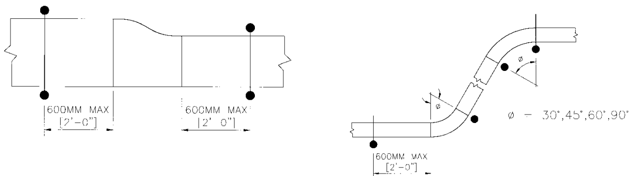
Figure 3-58 Reducer
