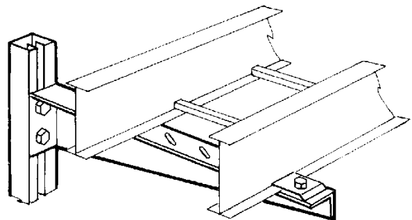
Figure 3-21 Gusset Cantilever Bracket
