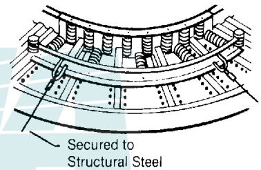
Figure 4-6 90° Roller Guide
