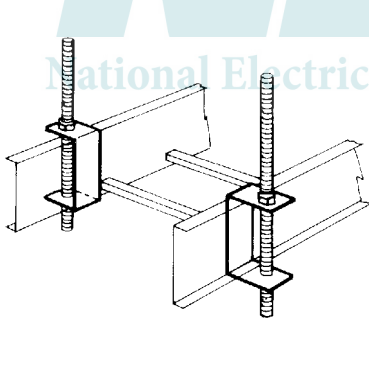
Figure 3-8 Single Cable Tray Hanger
