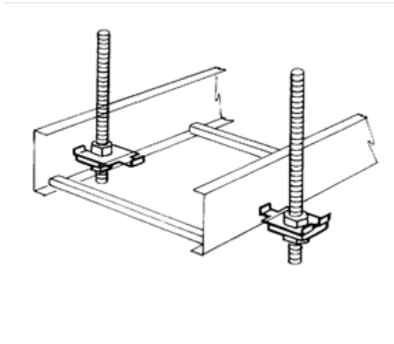
Figure 3-10 Single Cable Tray Hanger
